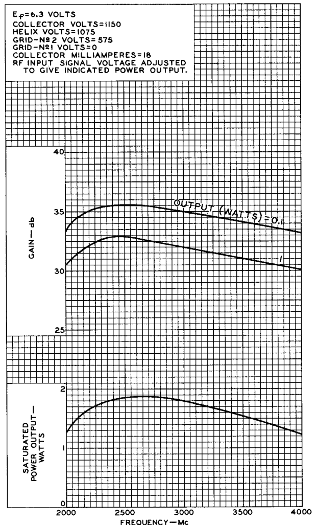
Fig. 4 - Typical Characteristics of Type 4010.
